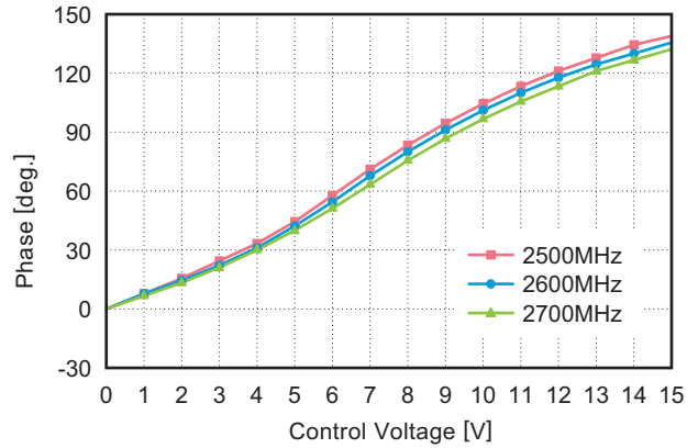
Control Voltage VS Phase
