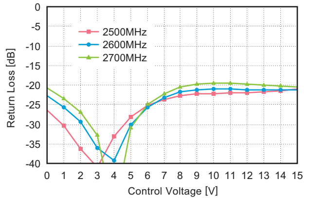
Control Voltage VS Return Loss (S11)
