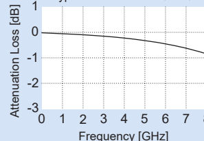
Typical Performance (TYP)
