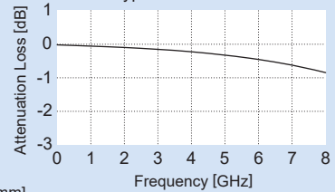
Typical Performance
