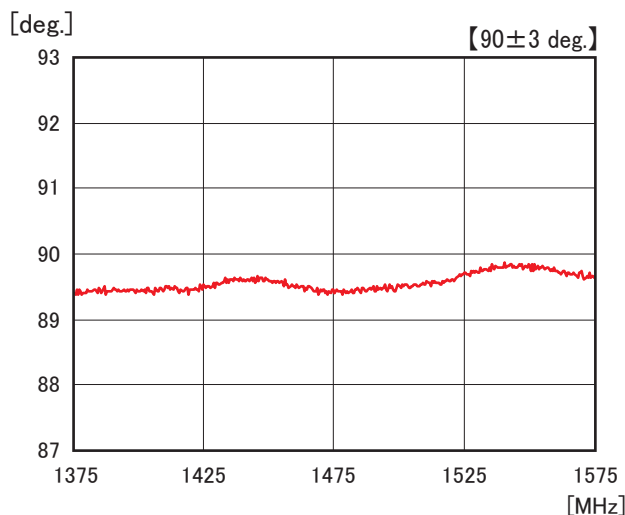
Phase Data
