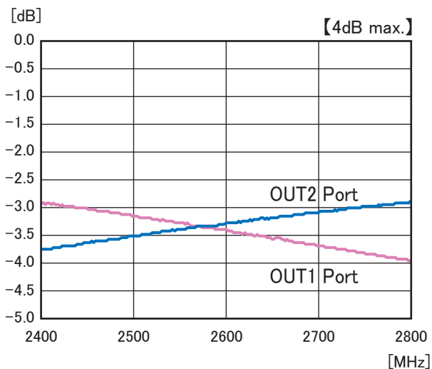
Insertion-Loss Data
