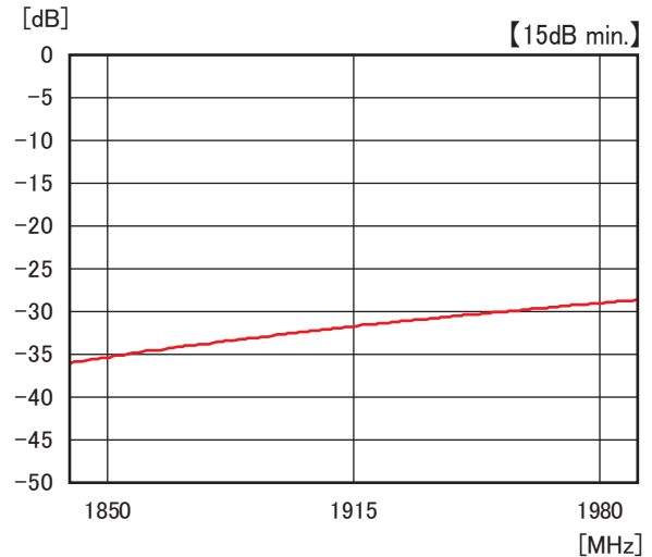
Isolation Data
