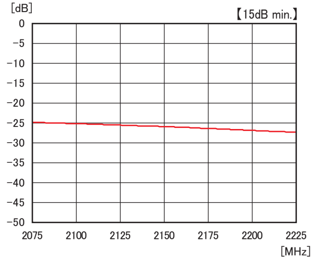
Isolation Data
