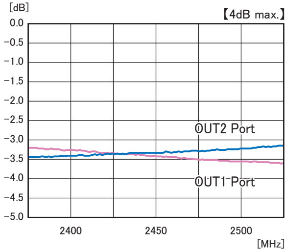
Insertion-Loss Data
