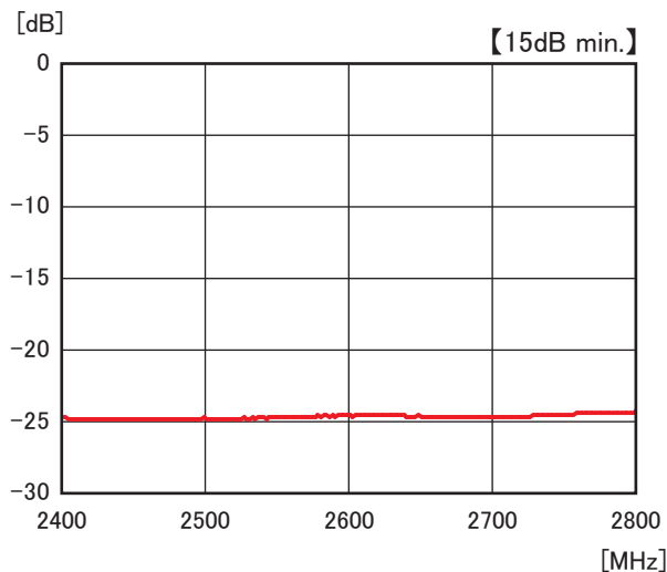
Isolation Data
