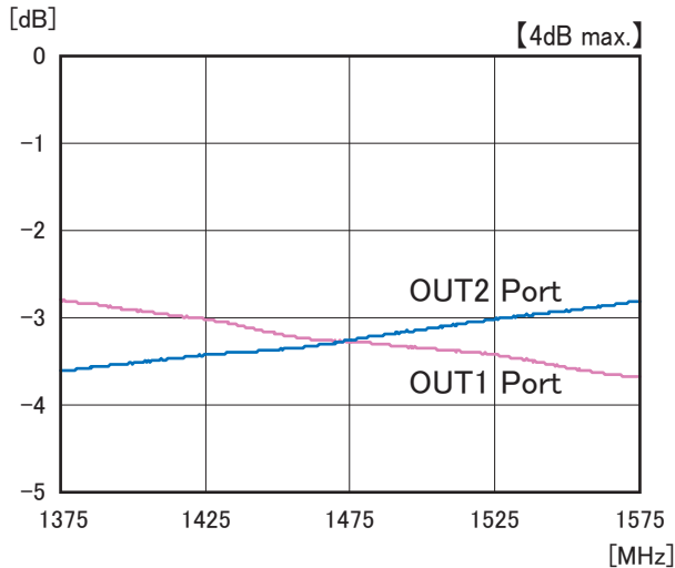
Insertion-Loss Data
