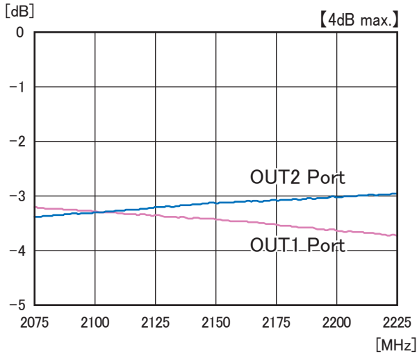
Insertion-Loss Data
