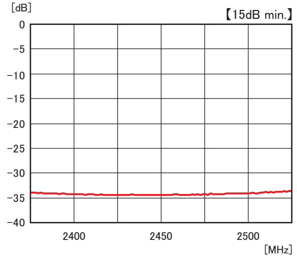
Isolation Data
