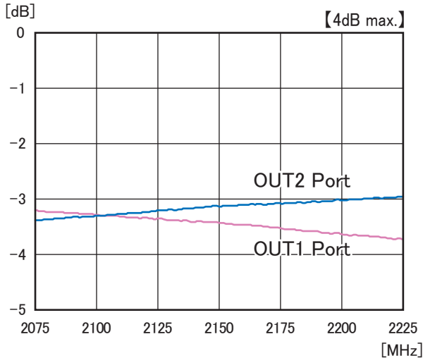
Insertion-Loss Data
