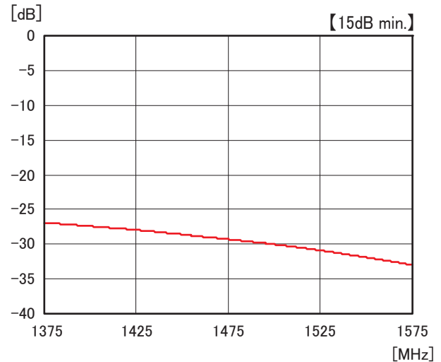
Isolation Data
