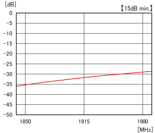
Isolation Data
