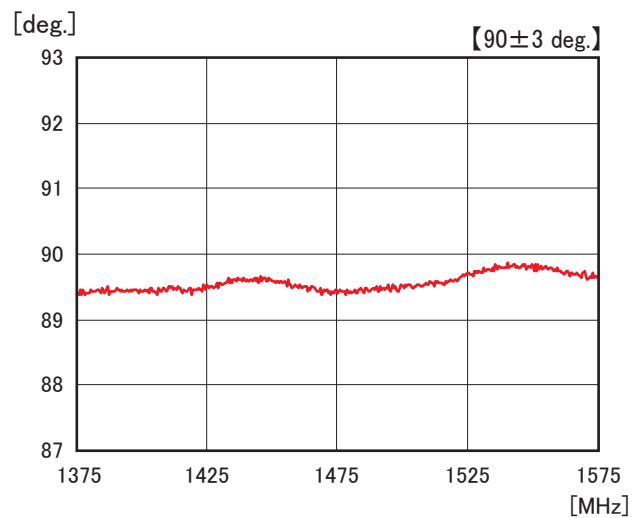
Phase Data
