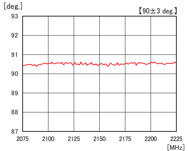
Phase Data
