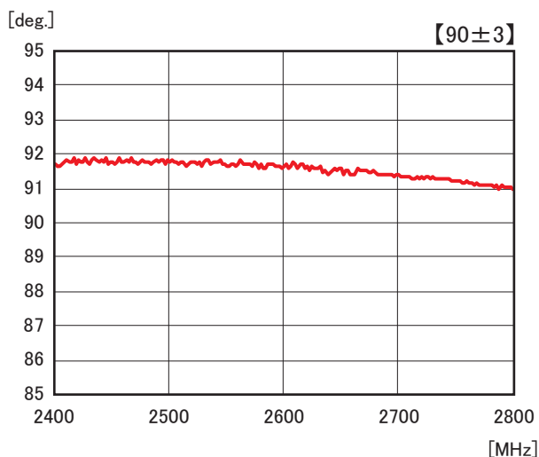
Phase Data
