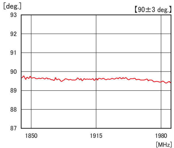
Phase Data
