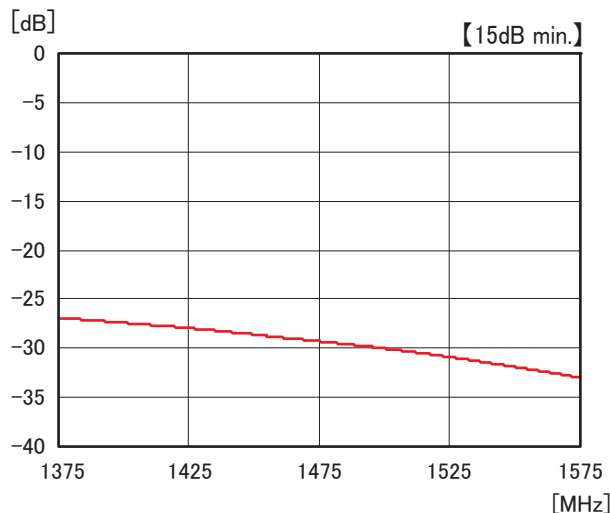
Isolation Data
