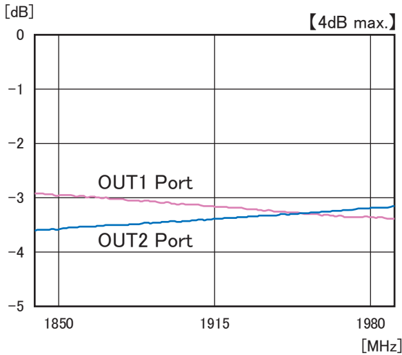
Insertion-Loss Data
